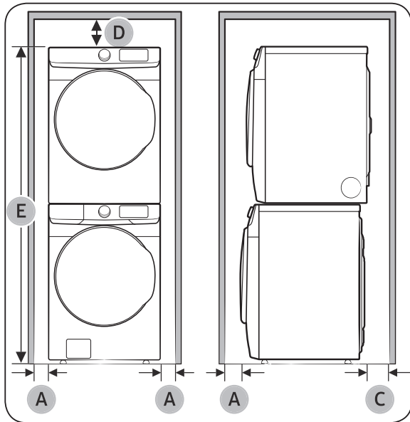
Stacked installation
