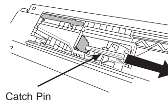
Catch Pin
