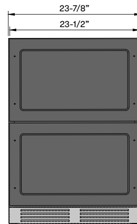
*Depth with 3/4" thick overlay panel ** Maximum clearance height inside drawers is 12"
