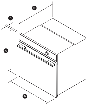
ISO VIEW
