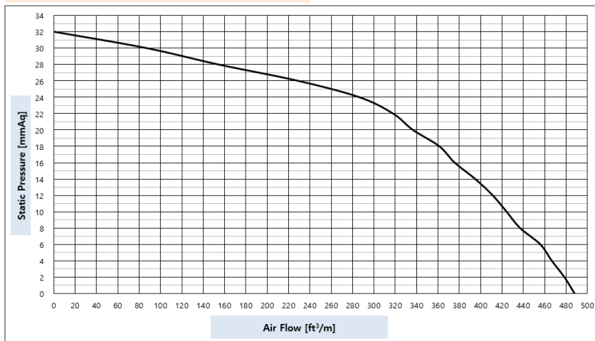
P-Q Curve(SMV-U480B1, Boost Mode)
