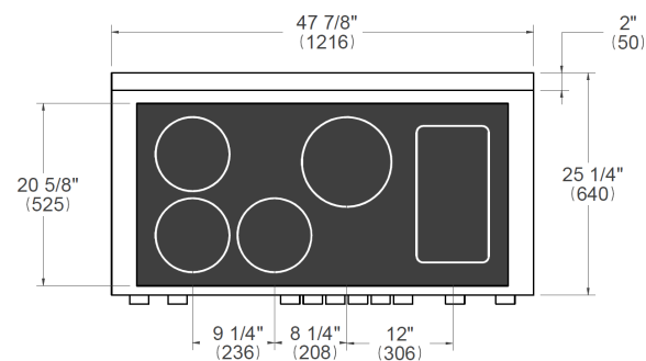
WORKTOP DETAILS
