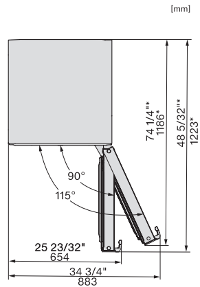
KFN4799DDE, top view (installation drawings) (US)
