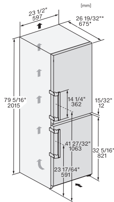
KFN4799DDE, installation sketch (footnote*) (installation drawings) (US)
