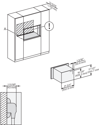
installation 30 inch Flush inset 450S, installation drawing, NA
