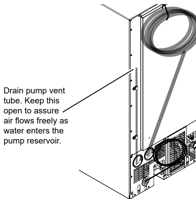
Location of vent tube.
