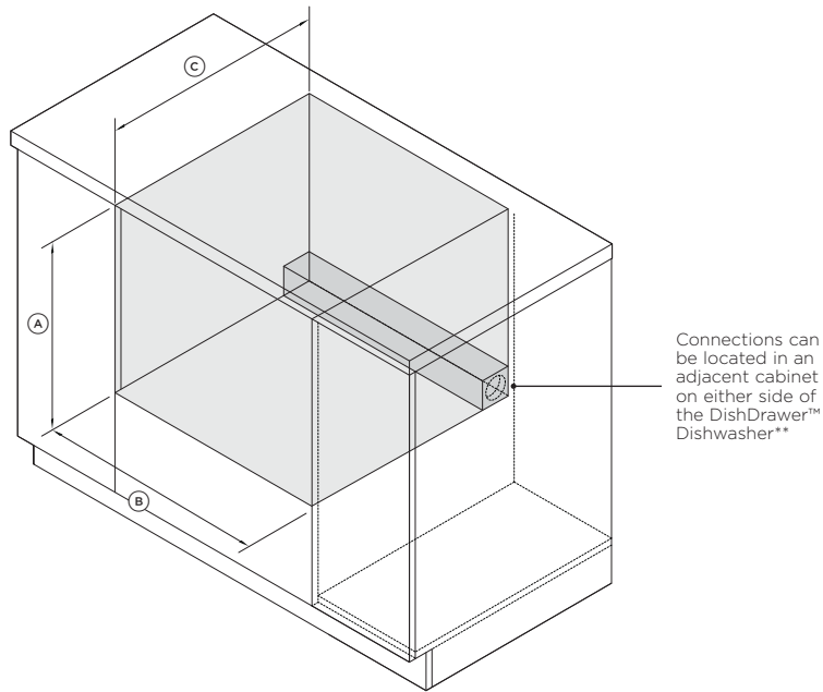
ISOMETRIC
