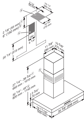
DA 6596 W (Installation drawing) – USA
