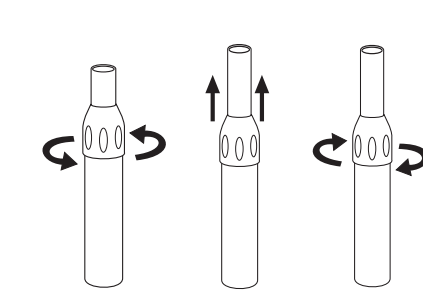
3. Loosen Nut, Extend Pipe Up, Tighten Nut
